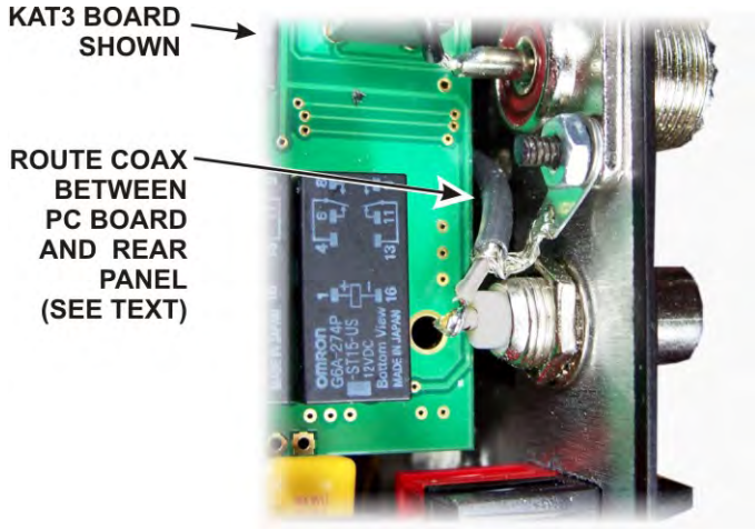
Figure 26. Routing AUX RF Connector Coax.
