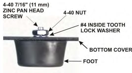
Figure 84. Installing Rear Feet.
