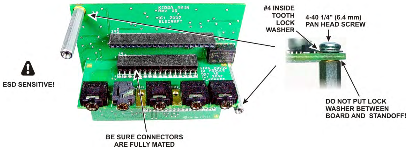
Figure 32. Preparing the KIO3 Board for Installation.
